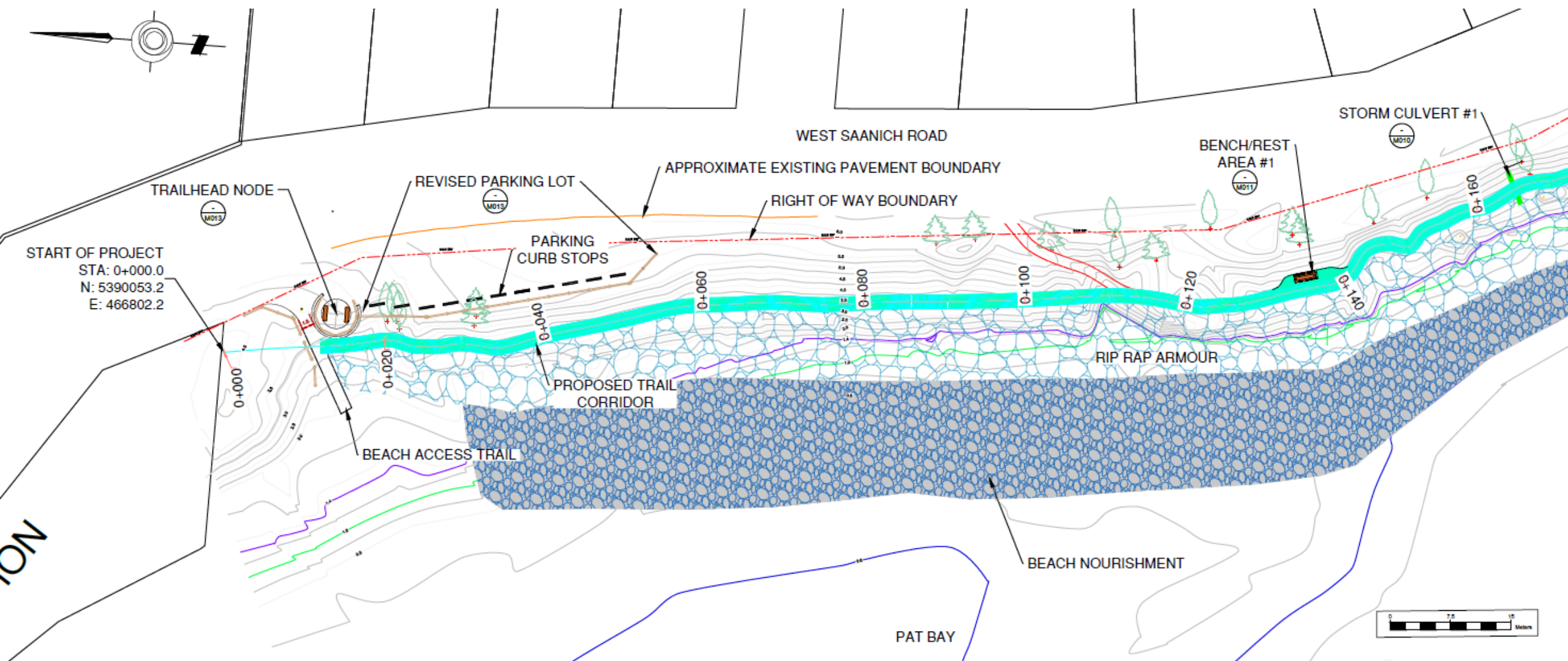
North Section of Project
