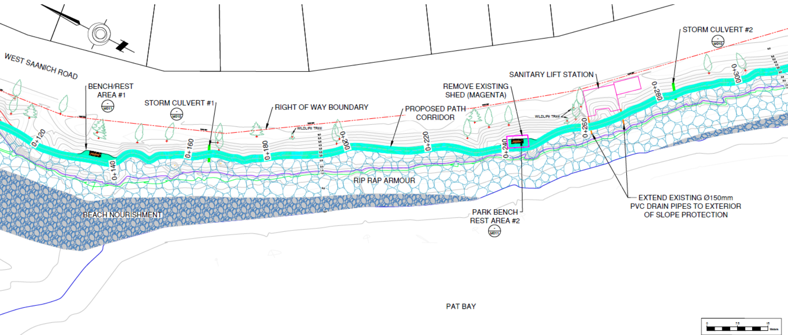
Middle Section of Project
